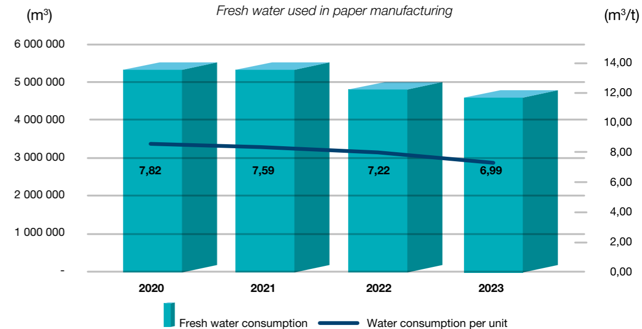
Fresh water used in paper manufacturing
